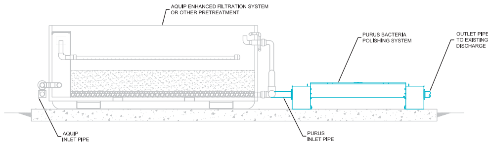
PURUS BACTERIA POLISHING – SECTION VIEW
